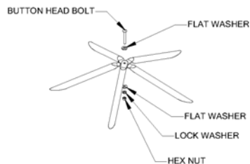
BOLTING DETAIL
