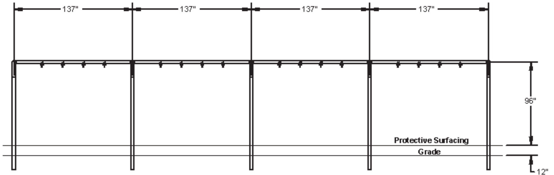
ELEVATION VIEW
