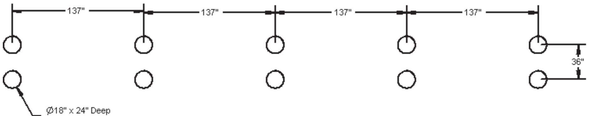
FOOTING LAYOUT
