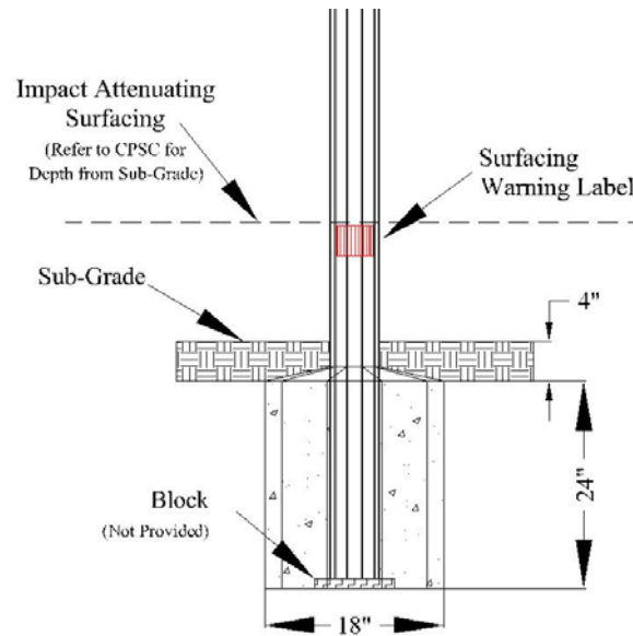
FOOTING ELEVATION
