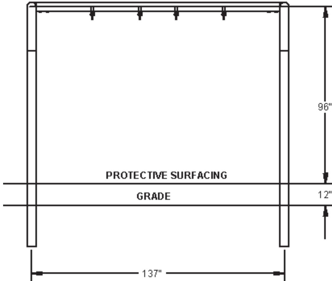
ELEVATION VIEW
