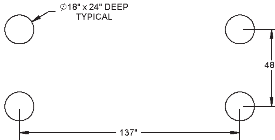
FOOTING LAYOUT
