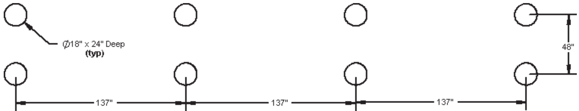
FOOTING LAYOUT
