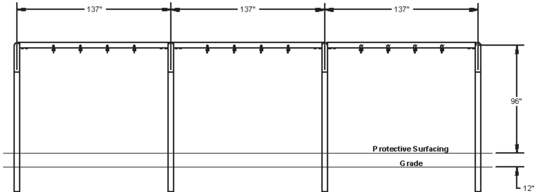
ELEVATION VIEW
