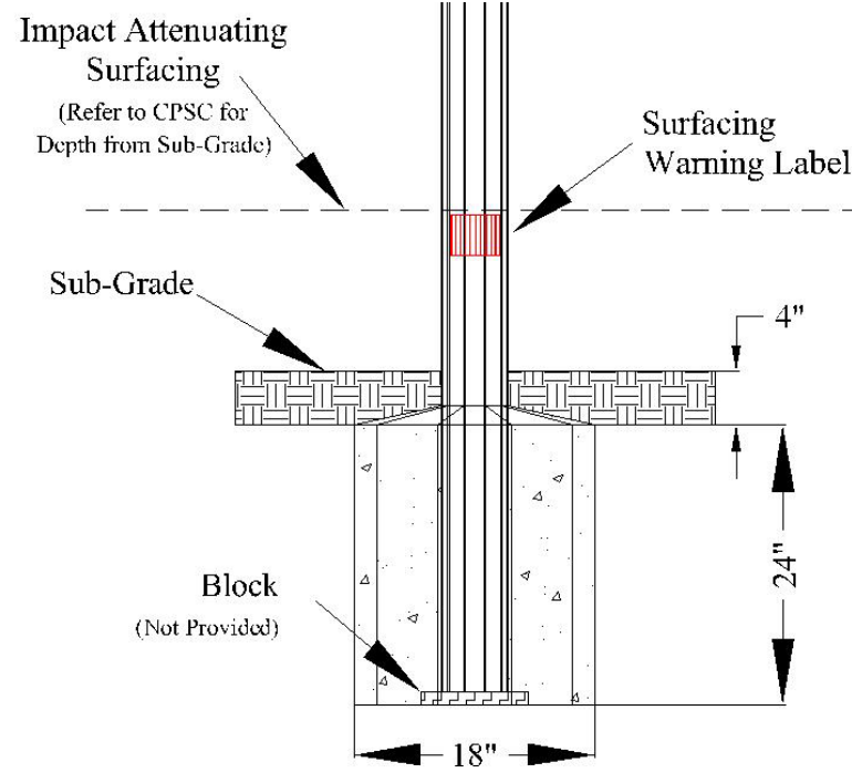
FOOTING ELEVATION
