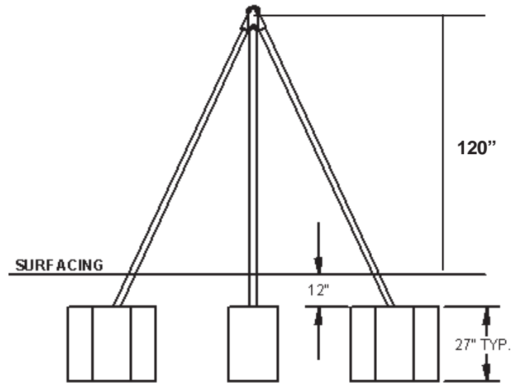
FOOTING DETAIL
