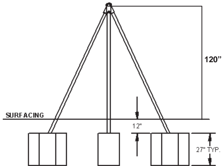
FOOTING DETAIL
