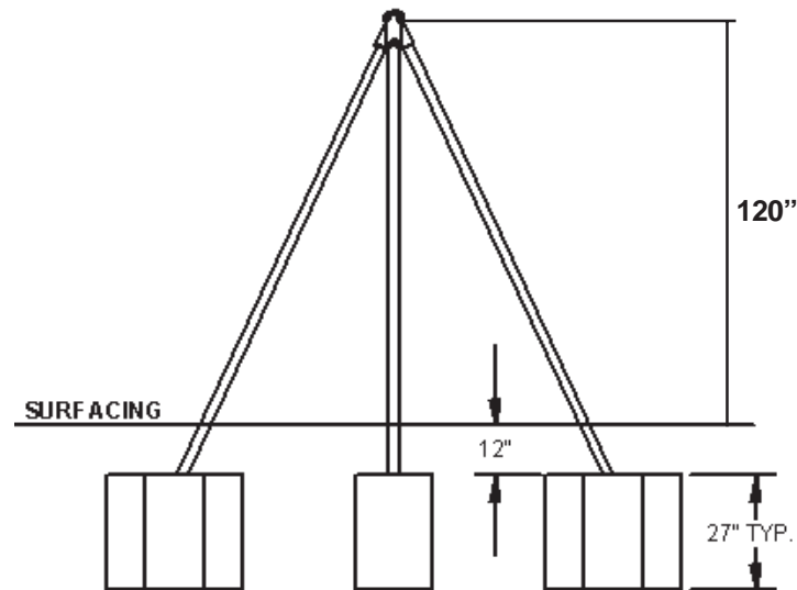
FOOTING DETAIL
