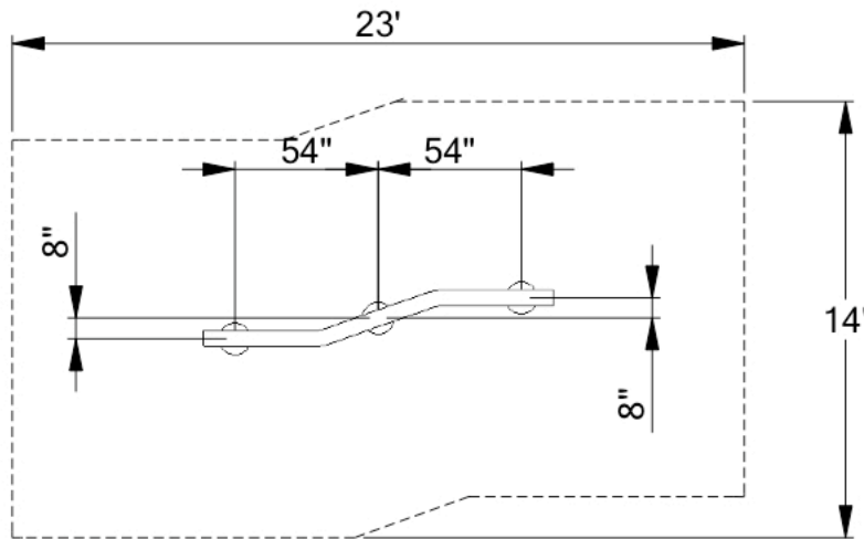
FOOTING DIAGRAM
