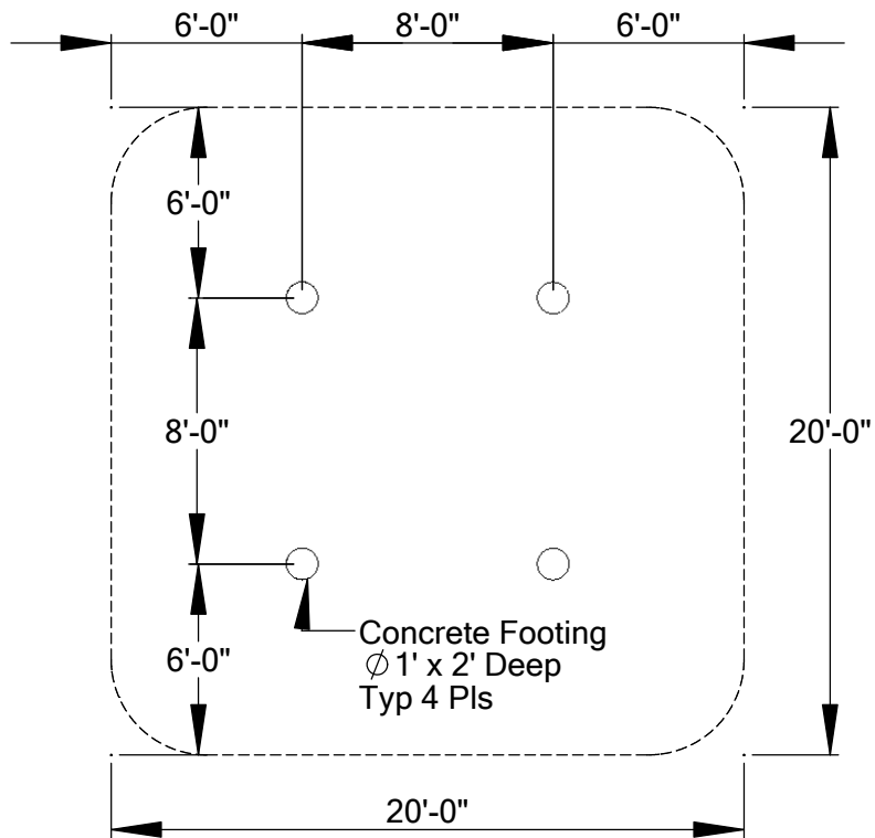
Footing Diagram
